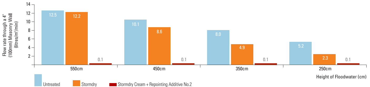
The reduction in waterflow through a wall after treatment with Stormdry Masonry Cream and Repointing Additive
